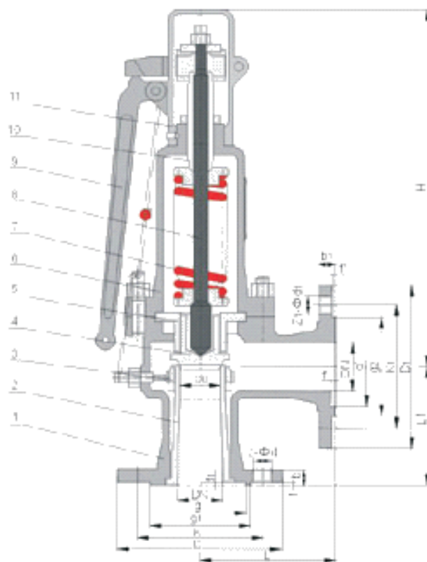
A47H Structural drawing
